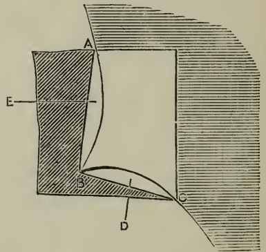
FIG. 179.—Diagram explaining the cutting of the corner blocks.
